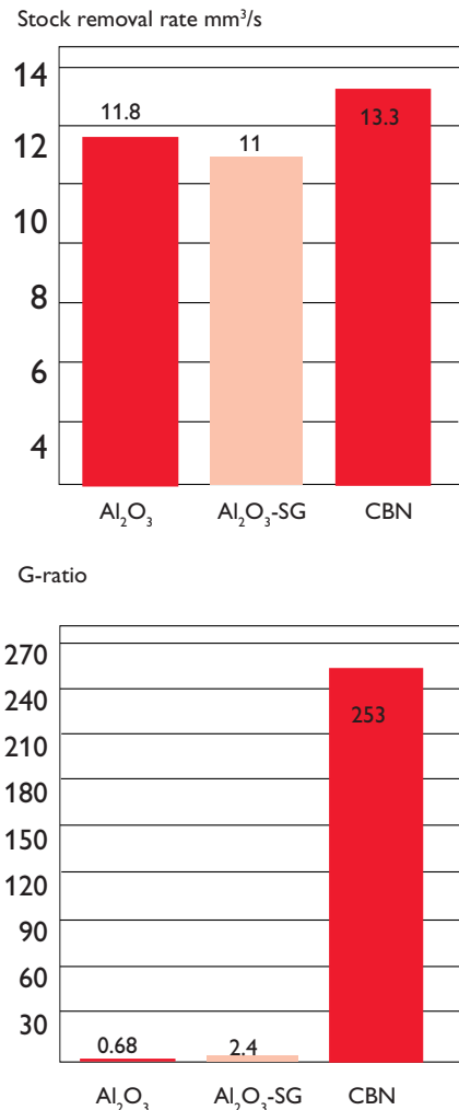
Figure 11. Surface grinding of Vanadis 10 SuperClean with various grinding wheels. (Grinding wheel width: Al 2 O 3 40 mm, CBN 20 mm.)
