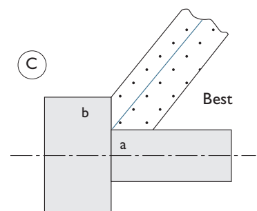
Figure 8. Incorrect grinding can often result in grinding cracks.
